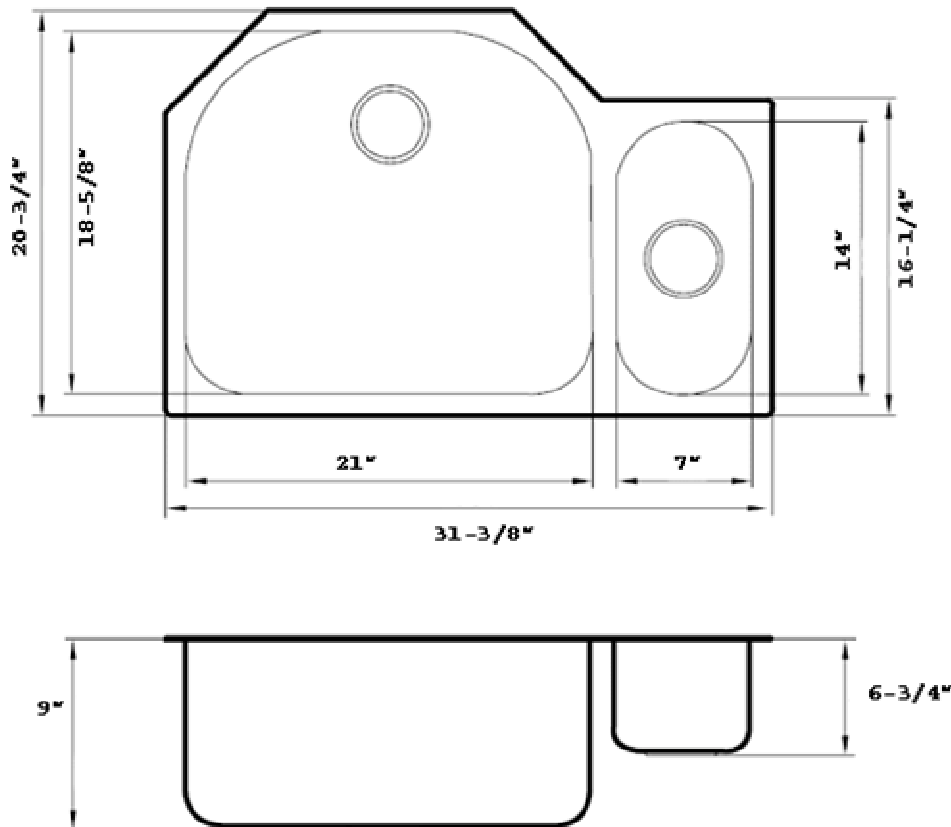
Dynasty Hardware 18 Gauge Stainless Steel Sink # 798-529
