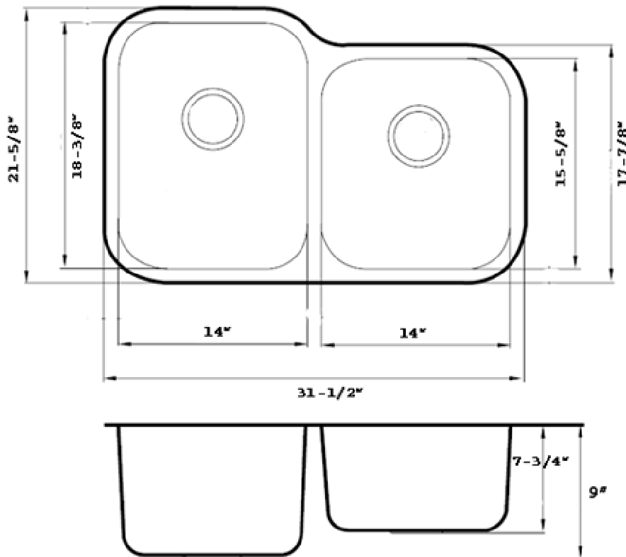
Dynasty 18 Gauge Stainless Steel Sink # 802-524
