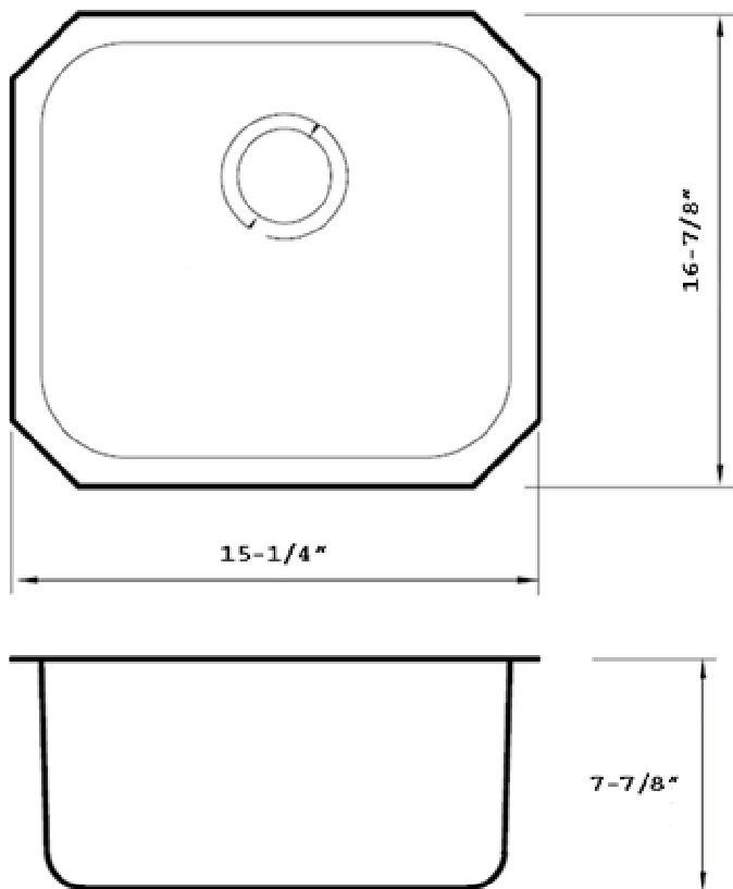
Dynasty 18 Gauge Stainless Steel Bar Sink # 100
