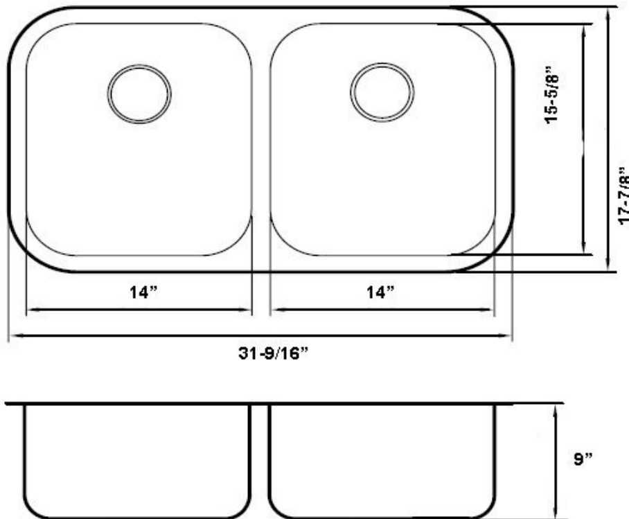
Dynasty 18 Gauge Stainless Steel Sink # 8400
