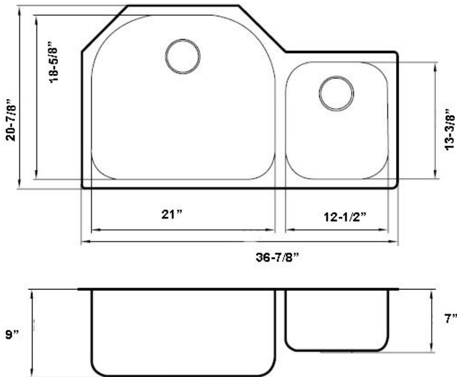
Dynasty 18 Gauge Stainless Steel Sink # 938-529
